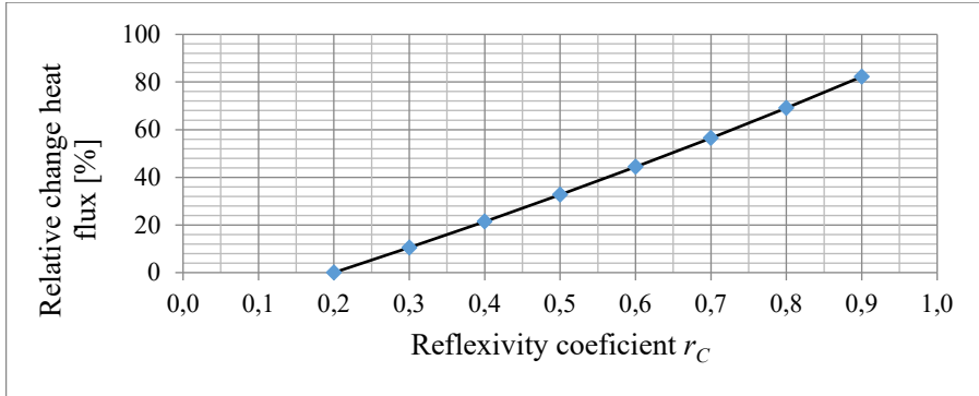
Fig.5. Per cent relative change of heat flux transferred to the interior through the roof with reflexivity coefficient for equivalent heat transfer coefficient equal 0,2 \text{ W}/(\text{m}^2\text{K})
