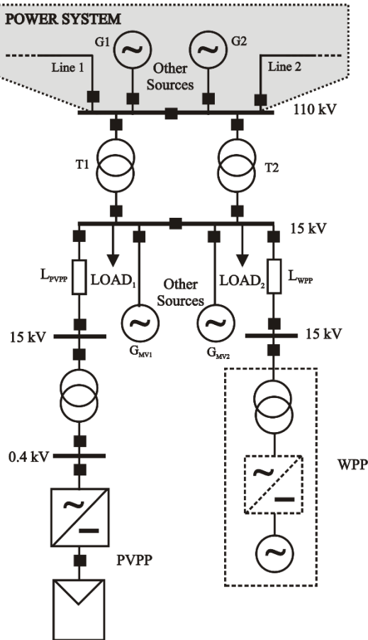
Fig. 1. Typical MV system with PVPP and WPP
